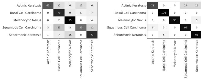
(a) CosSen CNN [24] (b) Affinity Loss Figure 4. Confusion matrices for Exp#1 on DIL dataset.
